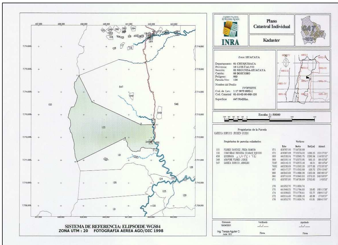
Figure 15 Fixed Boundaries with point identifiers, coordinates, distances between points and azimuth's; source INRA, Bolivia
