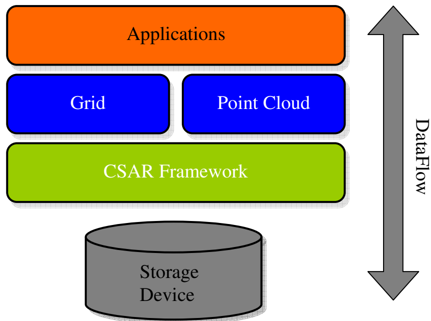
Figure 1: CARIS Application Technology Stack
